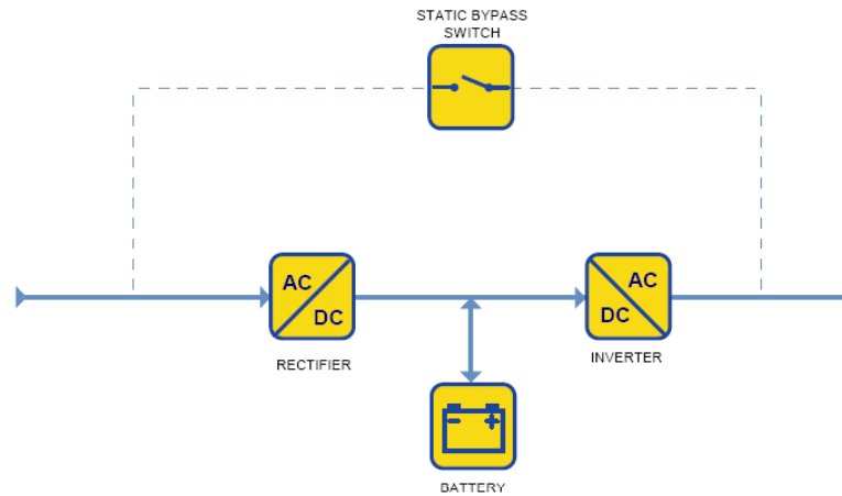
Figure 4 – Double Conversion On-Line UPS
