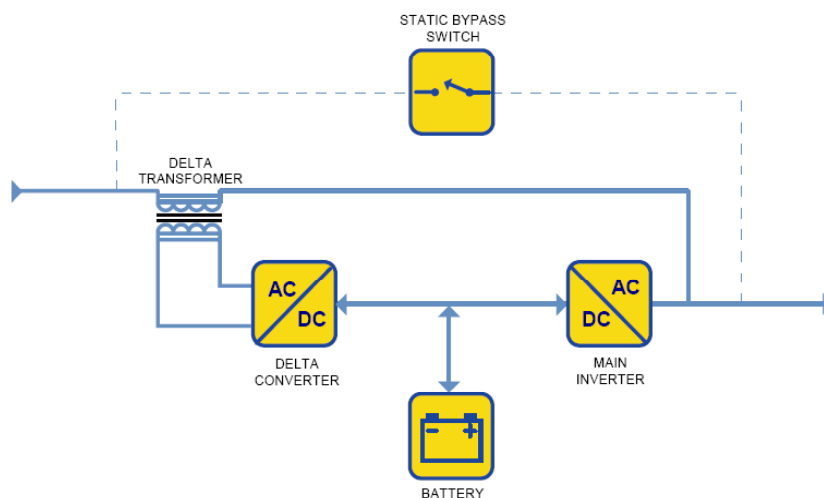
Figure 5 – Delta Conversion On-Line UPS
