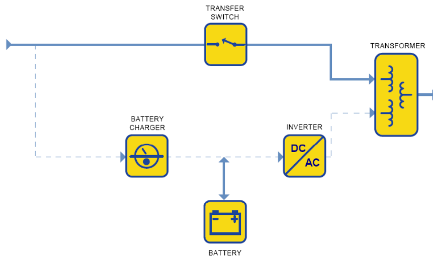
Figure 3 – Standby-Ferro UPS
